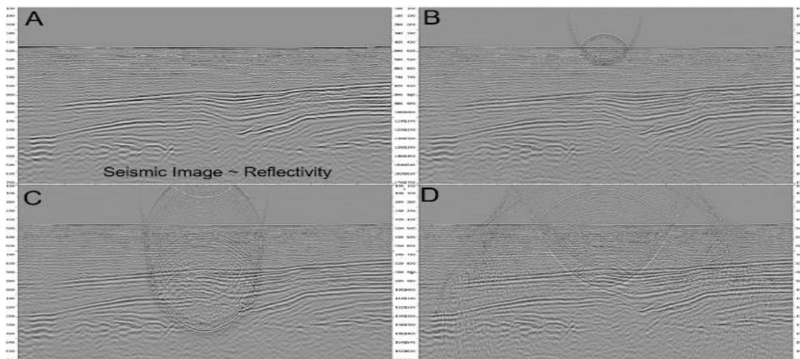
Figure 3 A. Seismic image (used as a reflectivity estimate) overlaying the reflectivity and modeled wavefield snapshots B, C, and D from the full wavefield reflectivity modeling for three different times
