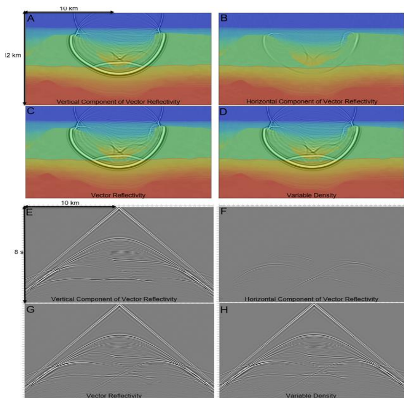
Figure 2 Seismic response for the model described in Figure 1. Displays A and E are a wavefield snapshot and surface seismogram using the vertical component of reflectivity. Displays B and F show the results using the horizontal component of reflectivity. Displays C and G are the results for vector reflectivity. Results using variable density modeling are shown in displays D and H.
