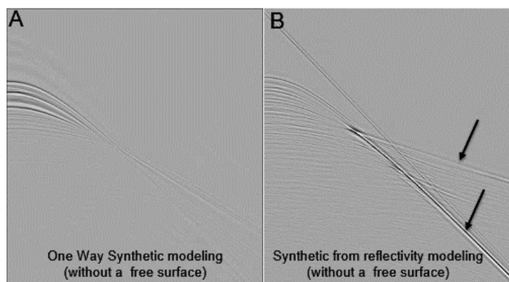
Figure 5 Comparison of one-way depth extrapolation synthetic (A) to the synthetic for the full wavefield reflectivity modeling (B). Note the refraction and high angle events in the full wavefield synthetic that are weak or absent in the one-way synthetic
