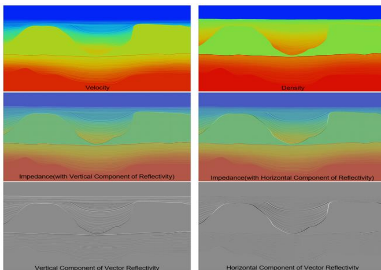
Figure 1. Model representation of a geological setting with the presence of salt. The top row shows the original velocity and density models. The second row shows the impedance for this model (with the vertical and horizontal components of the vector reflectivity interleaved). The third row shows the vertical and horizontal components of the vector reflectivity computed from the impedance.
